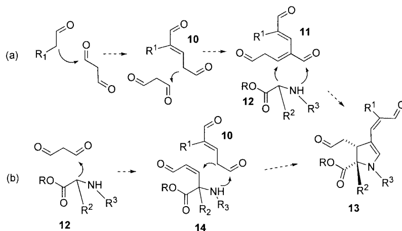
Scheme 3. Two possible pathways towards model intermediate 13 .
