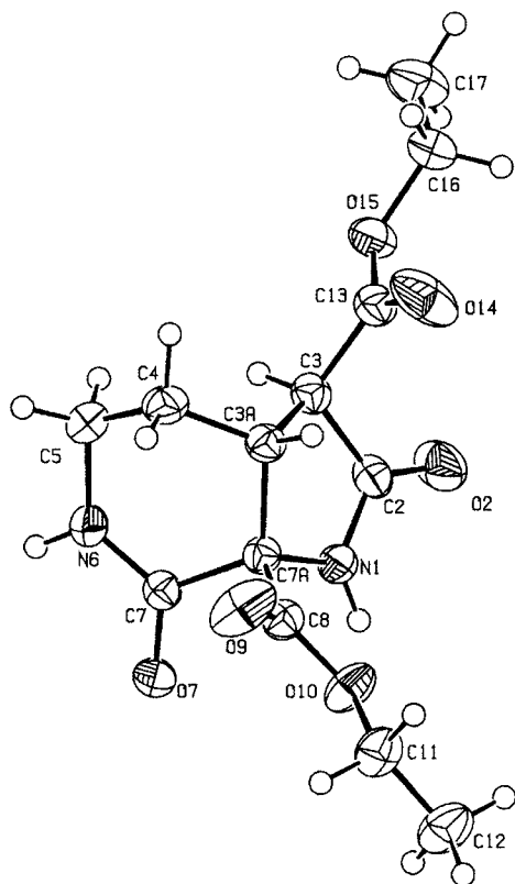
Figure 1. The molecular structure of pyrrolidinone 43 ; the displacement ellipsoids are plotted at the 50% probability level.
