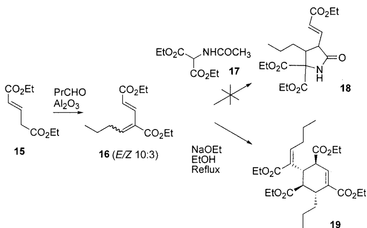
Scheme 3. Two possible pathways towards model intermediate 13 .
